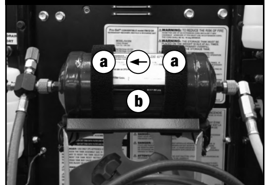
FIGURE - 2b Filter placed on filter bracket
