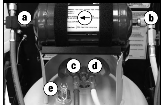
FIGURE - 2c Hose routing between filter, tank, and unit
